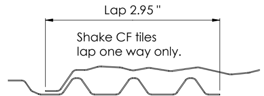
Figure 11.4 Side Lap Detail
