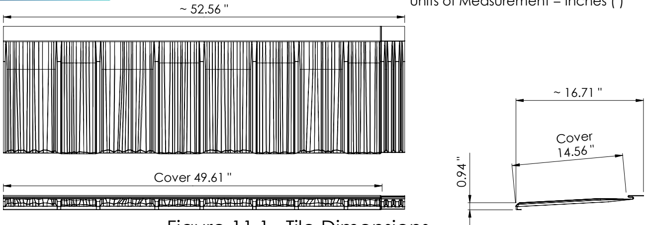
Figure 11.1 Tile Dimensions
