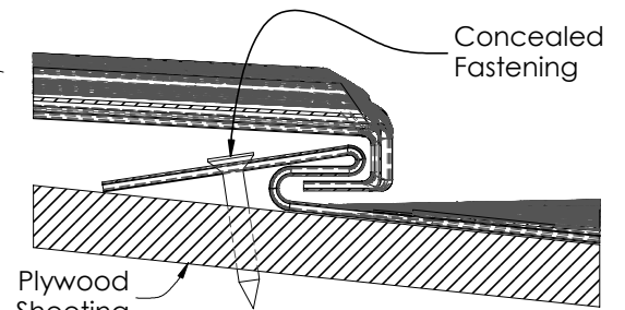
Figure 11.5 Nose Lap Detail
