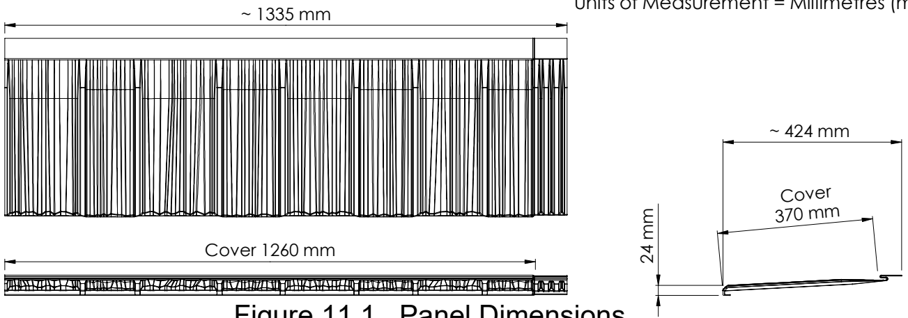
Figure 11.1 Panel Dimensions
