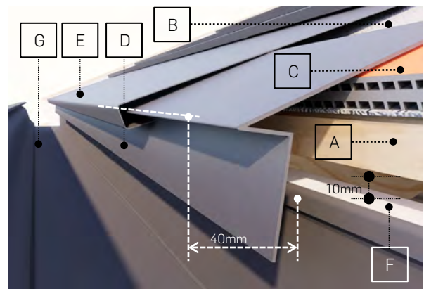
Color representation of ventilated batten
