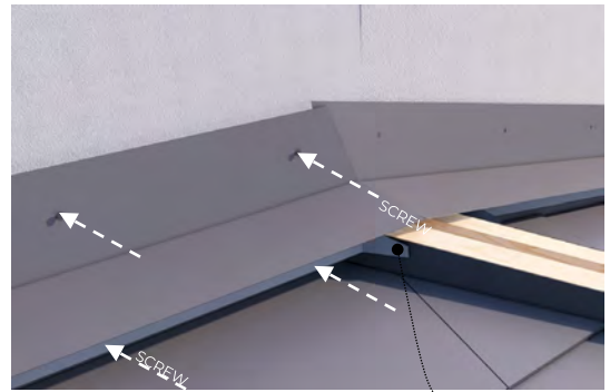
Bottom of the flashing folded parallel To the batten
