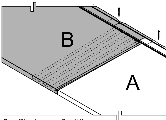
Overlap Detail
