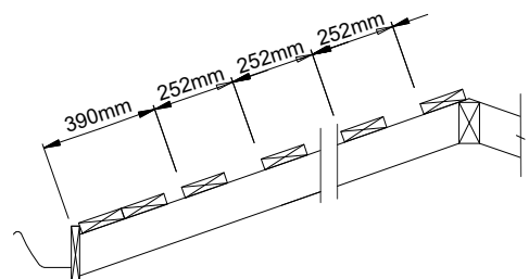
Batten Layout
